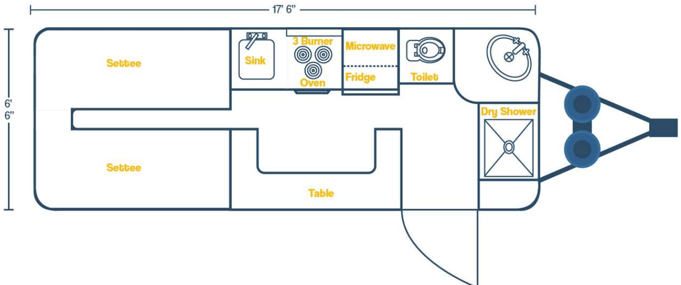
Cortes 22 DAY FLOOR PLAN Sleeps 3-4 (Dinette with Full Kitchen & Dry Bath)
